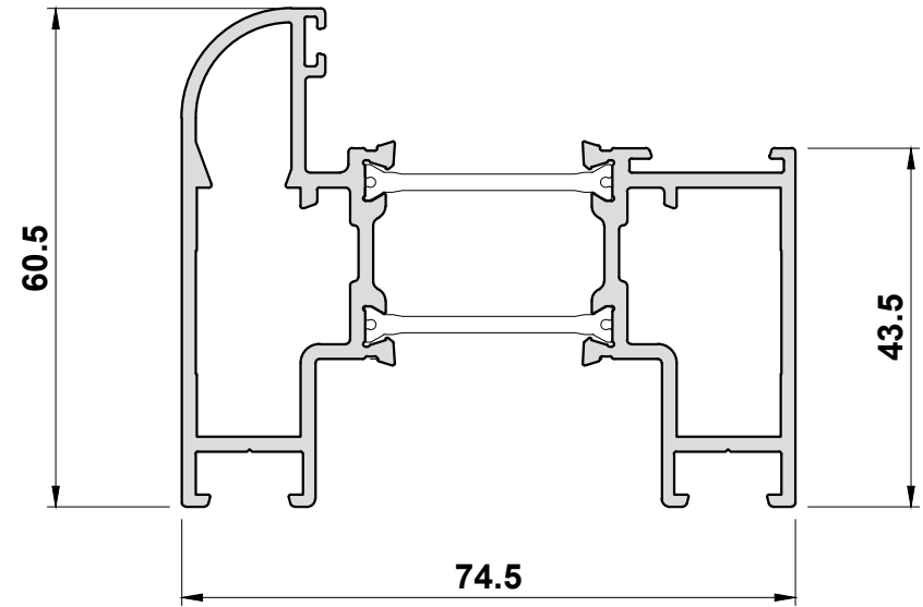
DV26 Curved Sash
